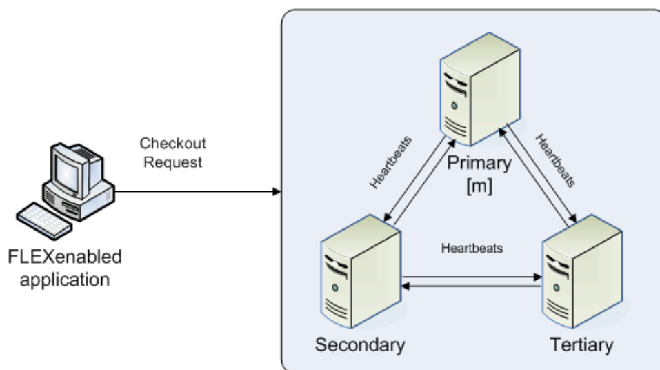
Figure 6-1: Three-Server Redundancy Overview
